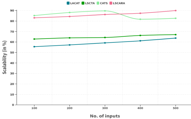
Fig.5 Comparison of Scalability
