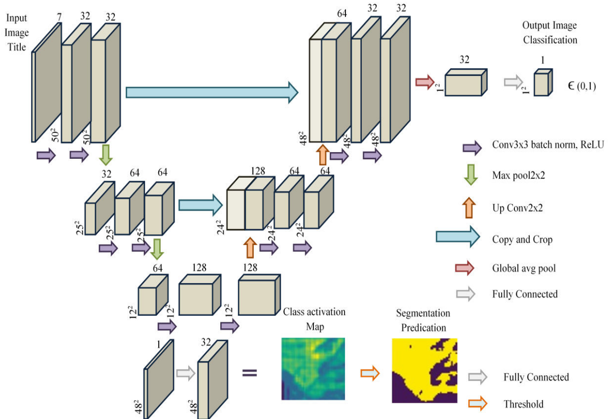
Fig 2 operating principle of the proposed model
