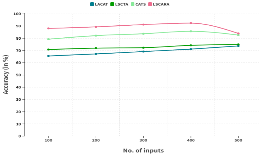
Fig.3 Comparison of Accuracy
