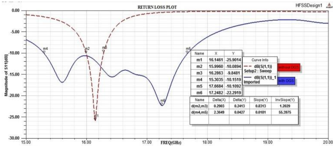
Figure 2 : Simulated reflection coefficient (in dB) of designs shown in Figure 1.
