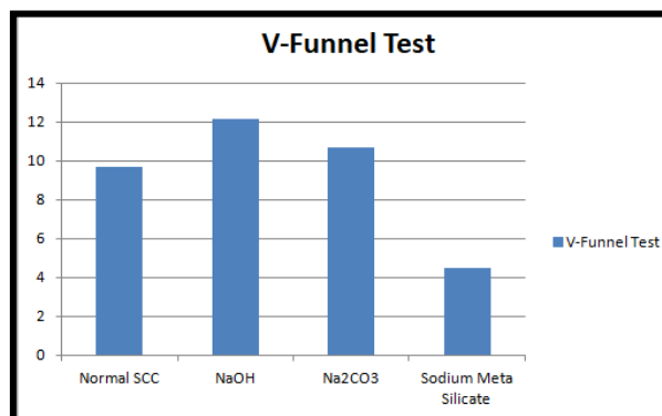
Graph 2: V Funnel Test Results ;
