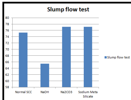
Graph 1: Slump Cone Test Results ;
