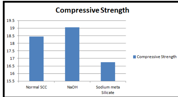
Graph 3: Compressive Strength Results ;
