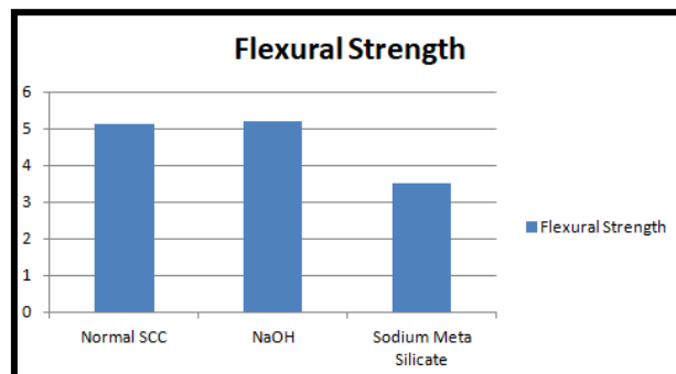
Graph 5: Flexural Strength Results .
