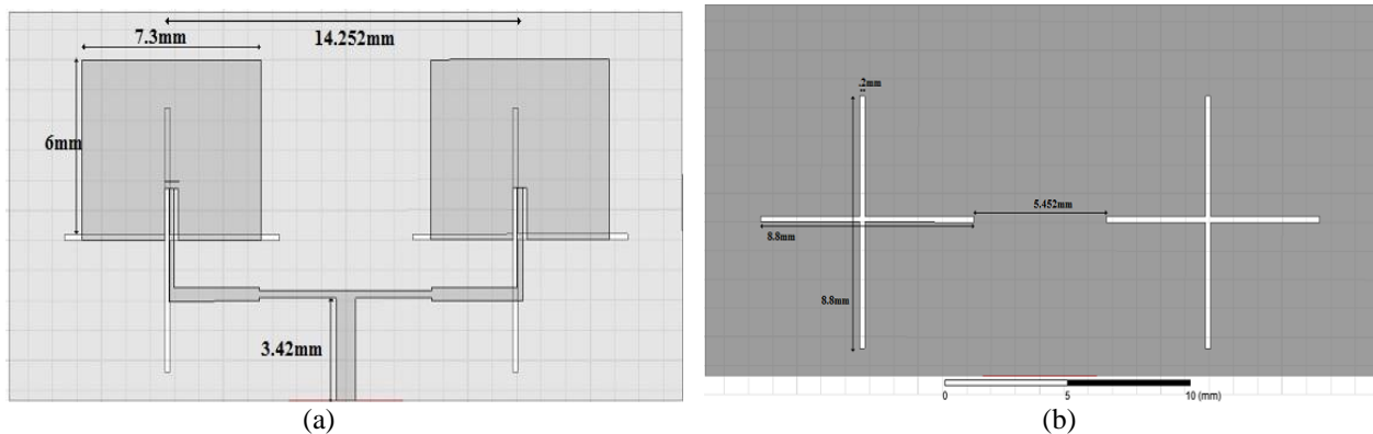
Figure 1: (a) Geometry of 1×2 Rectangular array with Cross slots in Ground Plane (Top view) , (b) cross slots in ground plane (bottom view).
