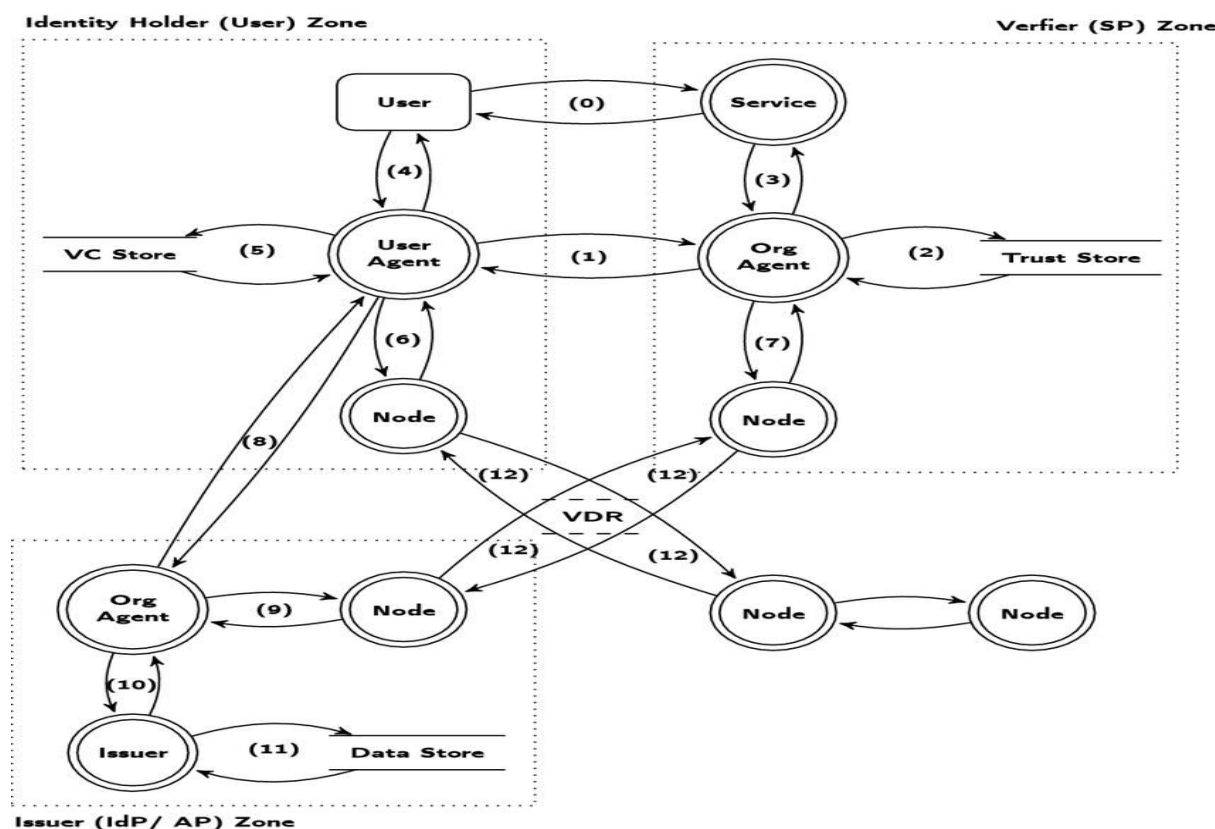
Figure 1: Blockchain-Based Digital Identity Flow
